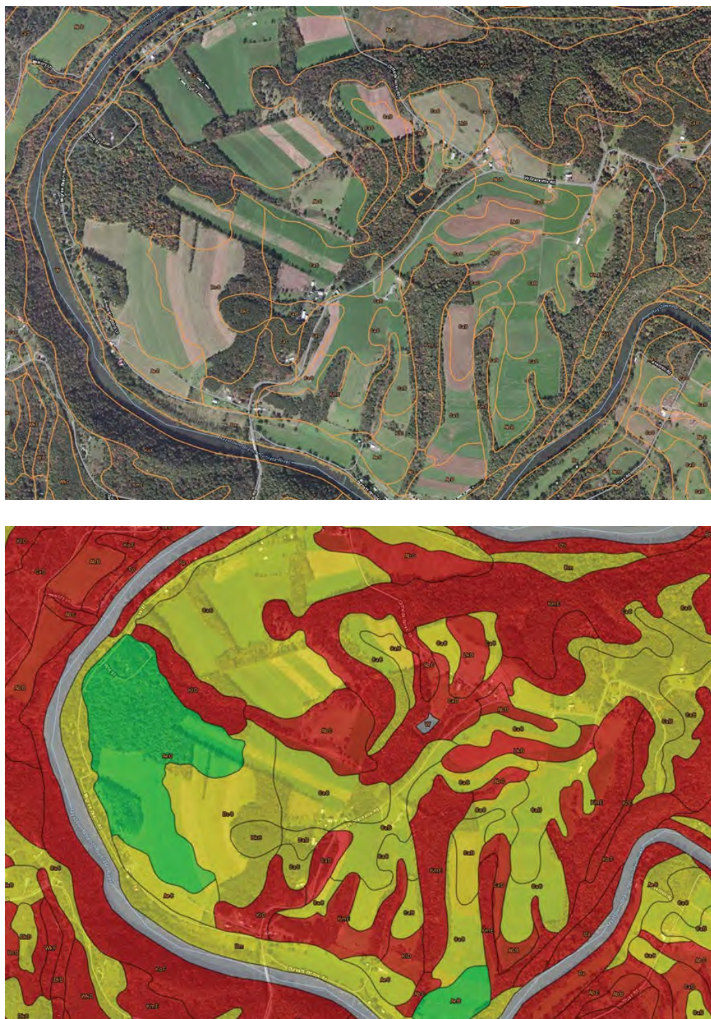
Soil map (top) showing the distribution of mapping units on the landscape and interpretive map (bottom) showing limitations for local roads and streets.
